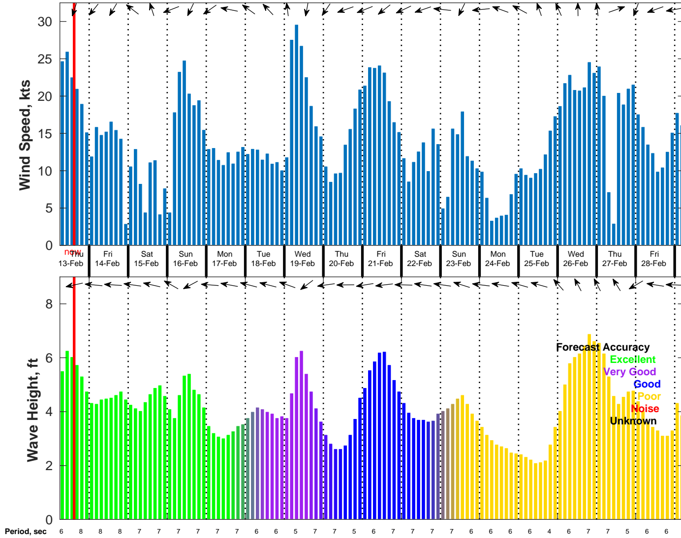
Wind & Wave Forecast for NDBC 42092 from 13-Feb-2025 06:00:00 to 01-Mar-2025 06:00:00
