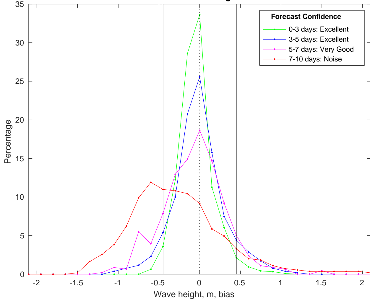
NDBC 46011 vs CMEMS Waves Bias Histogram: 13-Feb-2025
