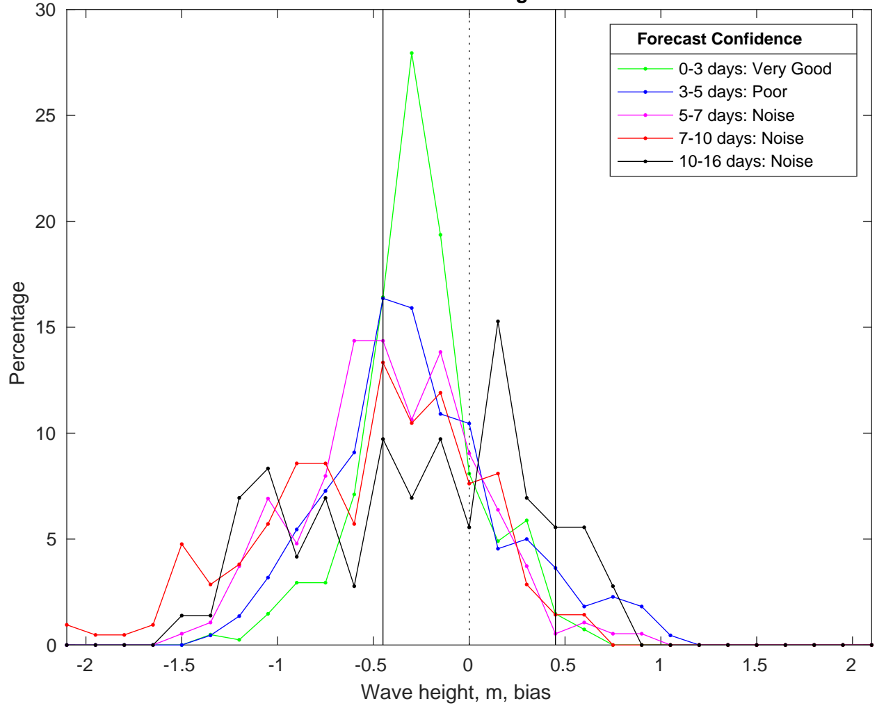
NDBC 46028 vs GFS Waves Bias Histogram: 13-Feb-2025
