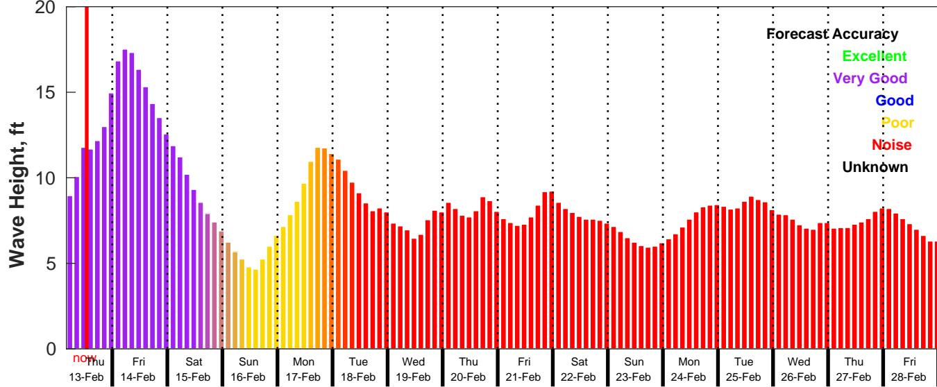
GFS Wave Forecast for NDBC 46028 from 13-Feb-2025 04:00:00 to 01-Mar-2025 04:00:00
