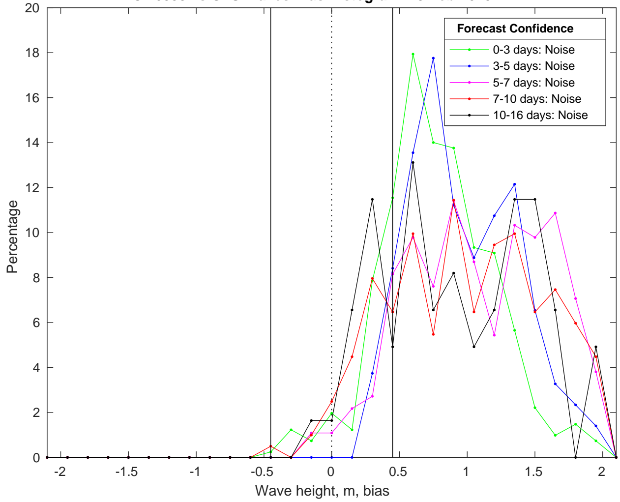
NDBC 46053 vs GFS Waves Bias Histogram: 13-Feb-2025
