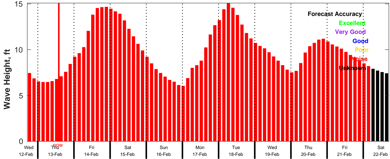
CMEMS Wave Forecast for NDBC 46053 from 12-Feb-2025 17:00:00 to 22-Feb-2025 17:00:00
