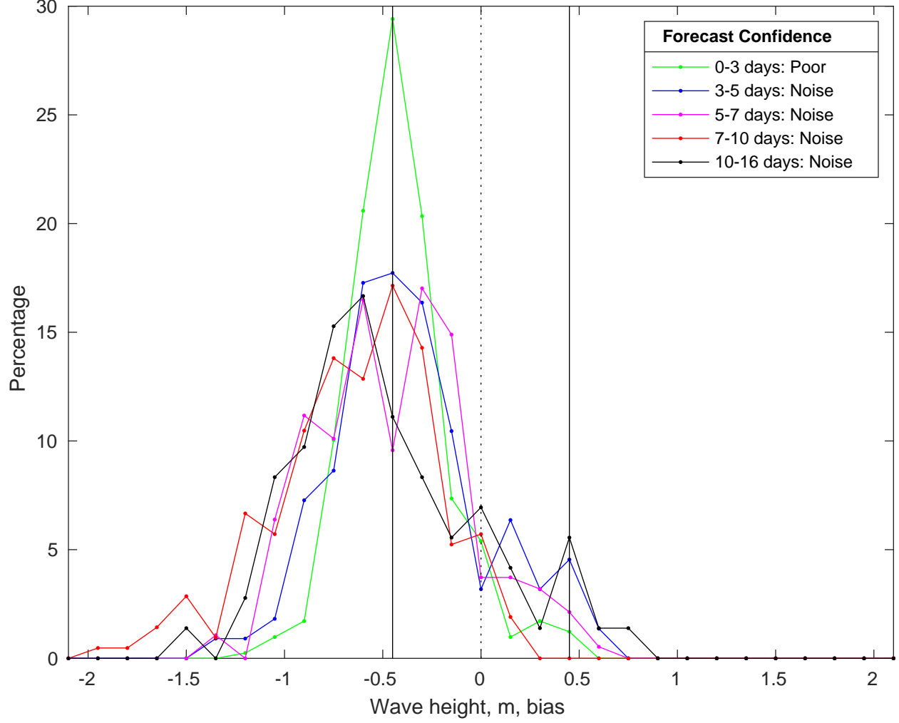
NDBC 46054 vs GFS Waves Bias Histogram: 13-Feb-2025
