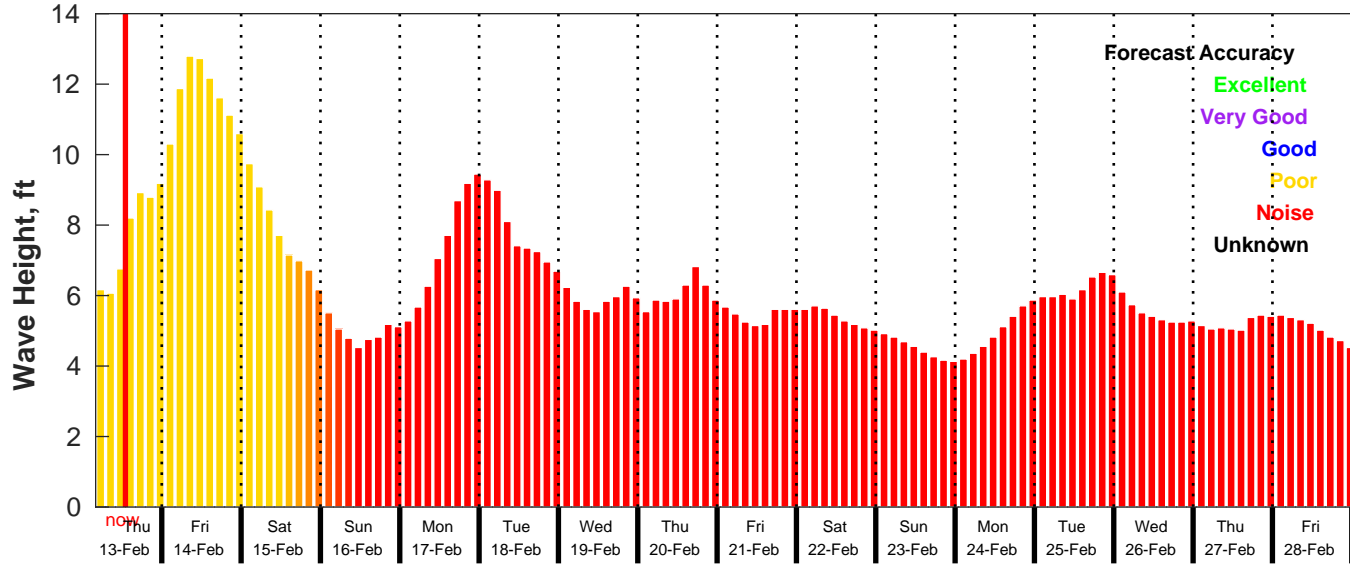
GFS Wave Forecast for NDBC 46054 from 13-Feb-2025 04:00:00 to 01-Mar-2025 04:00:00
