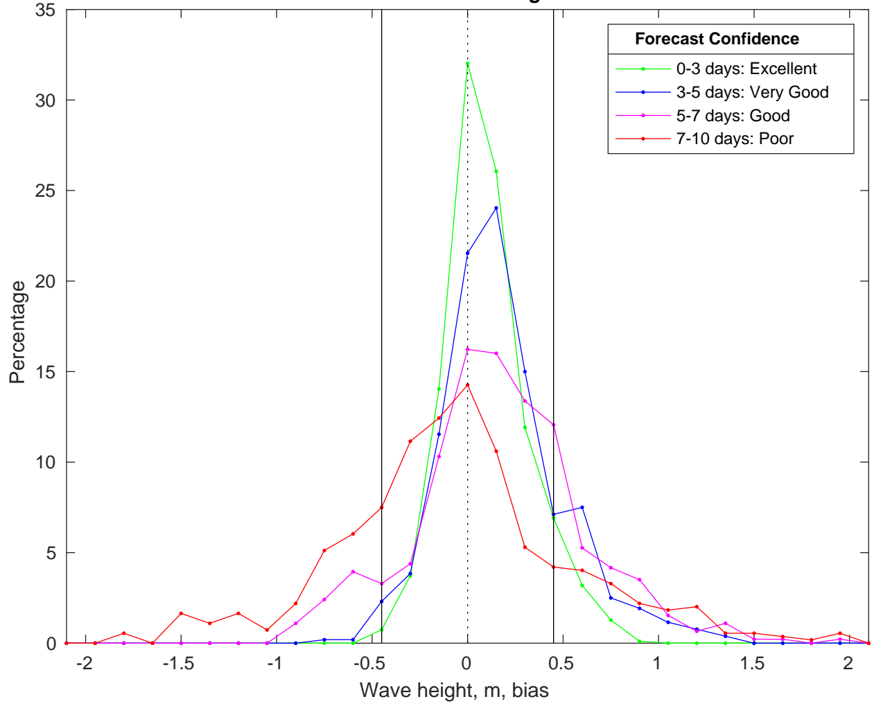
NDBC 46069 vs CMEMS Waves Bias Histogram: 13-Feb-2025
