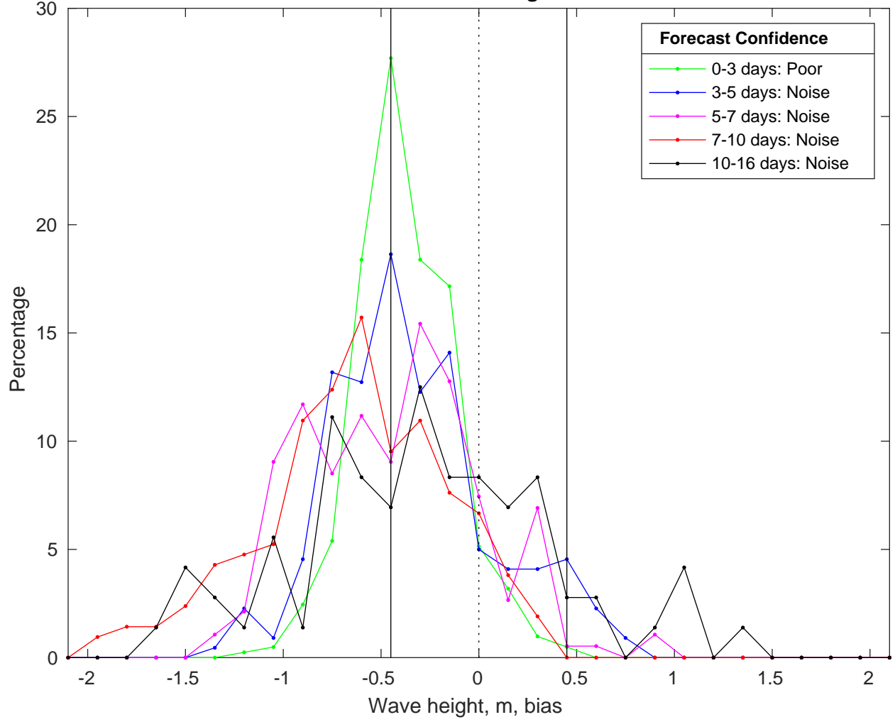
NDBC 46069 vs GFS Waves Bias Histogram: 13-Feb-2025
