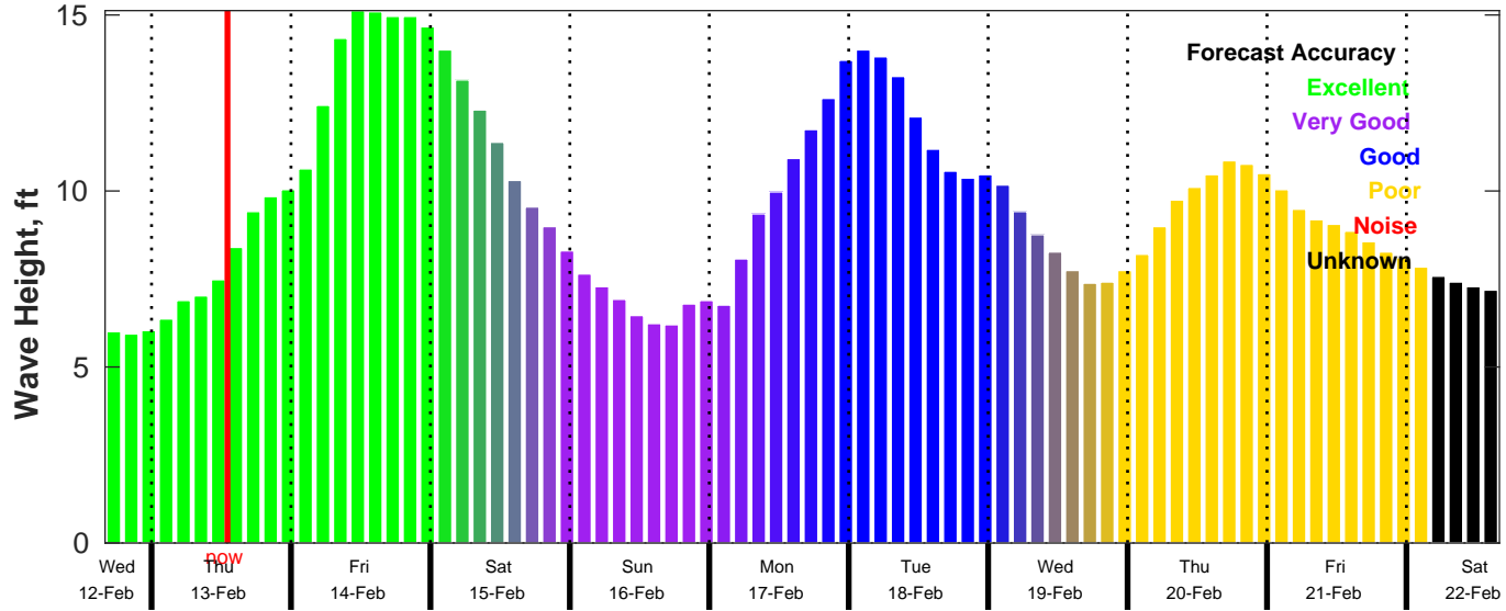
CMEMS Wave Forecast for NDBC 46069 from 12-Feb-2025 16:00:00 to 22-Feb-2025 16:00:00
