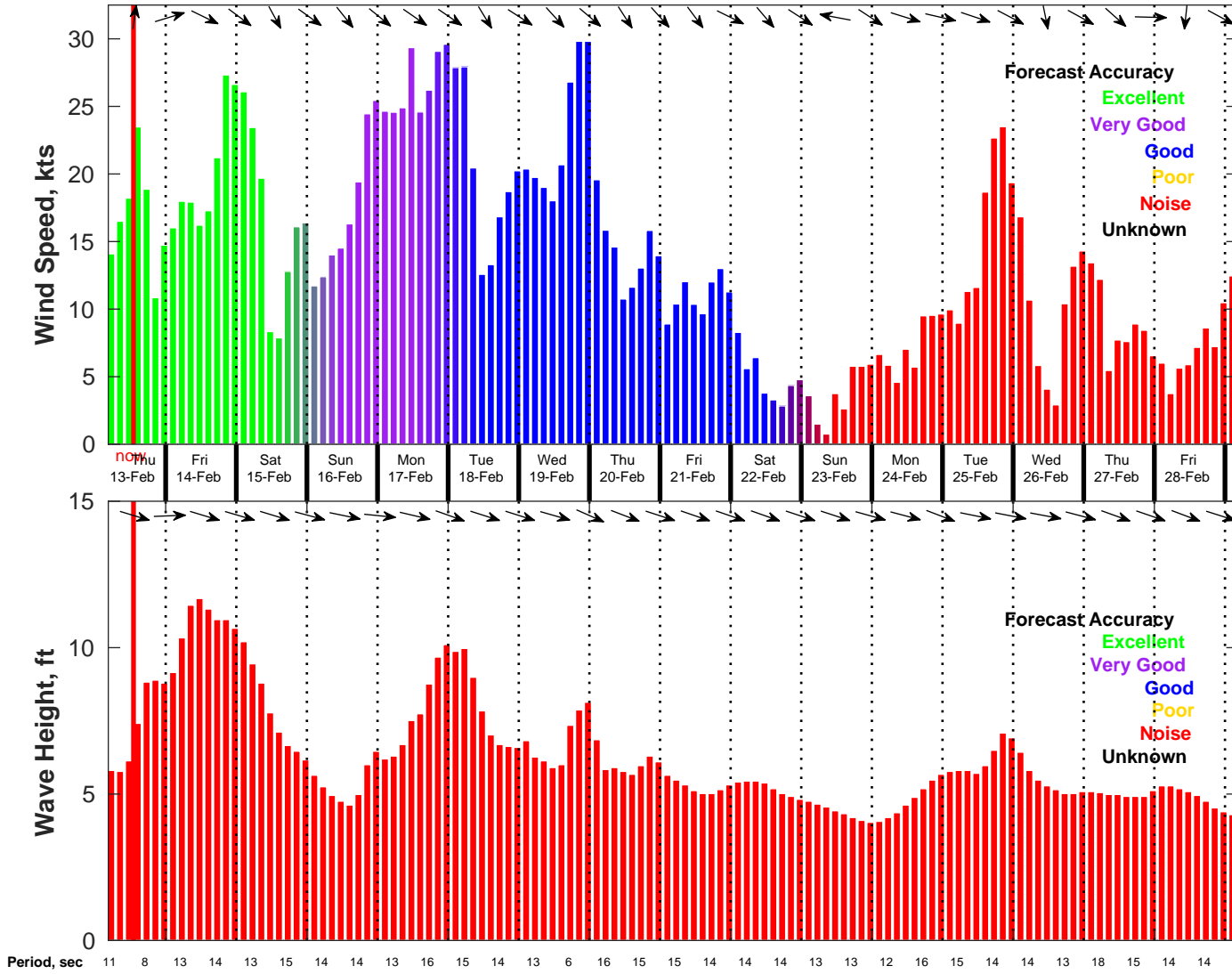
Wind & Wave Forecast for NDBC 46069 from 13-Feb-2025 04:00:00 to 01-Mar-2025 04:00:00
