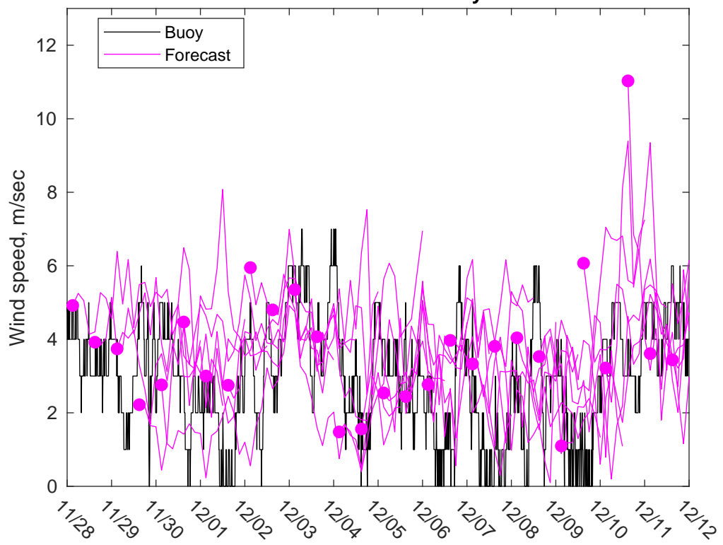
NDBC 46086 vs GFSWinds: 7 to 10 day forecast
