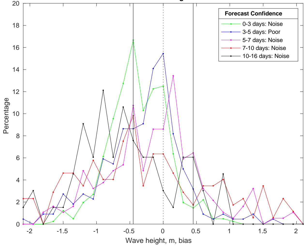
NDBC 46246 vs GFS Waves Bias Histogram: 13-Feb-2025
