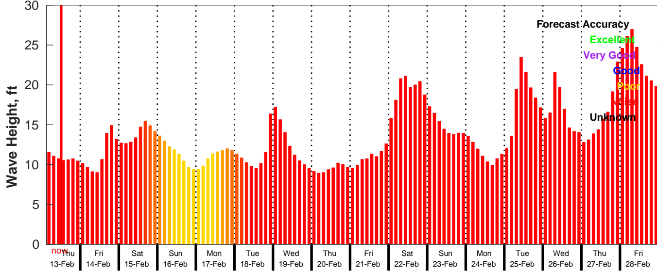
GFS Wave Forecast for NDBC 46246 from 13-Feb-2025 03:00:00 to 01-Mar-2025 03:00:00
