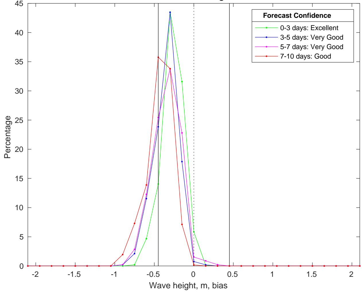
NDBC 51209 vs CMEMS Waves Bias Histogram: 13-Feb-2025
