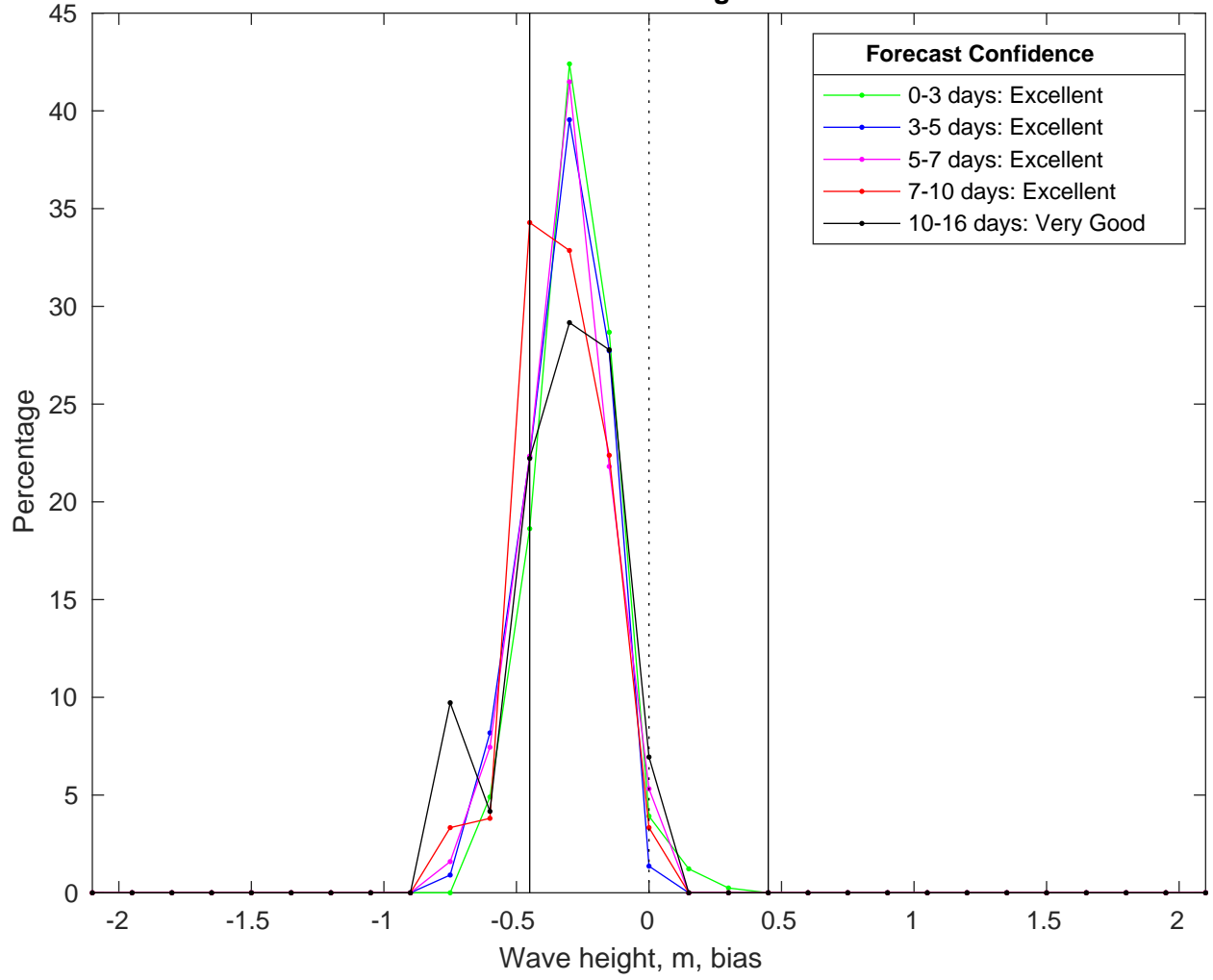
NDBC 51209 vs GFS Waves Bias Histogram: 13-Feb-2025
