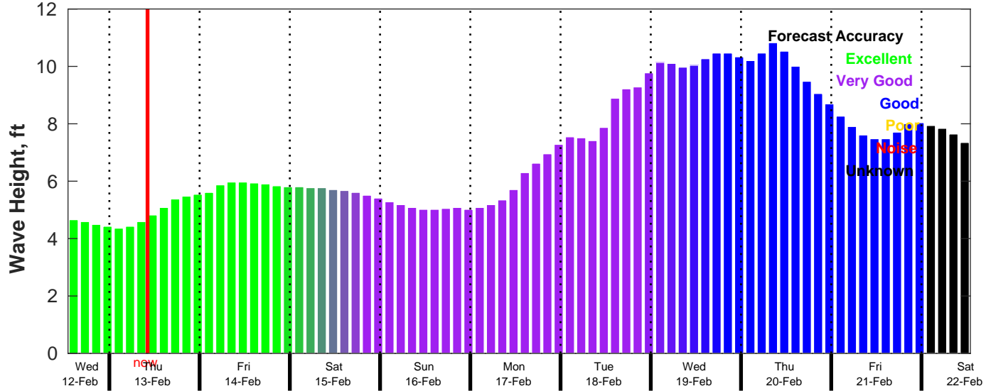
CMEMS Wave Forecast for NDBC 51209 from 12-Feb-2025 13:00:00 to 22-Feb-2025 13:00:00
