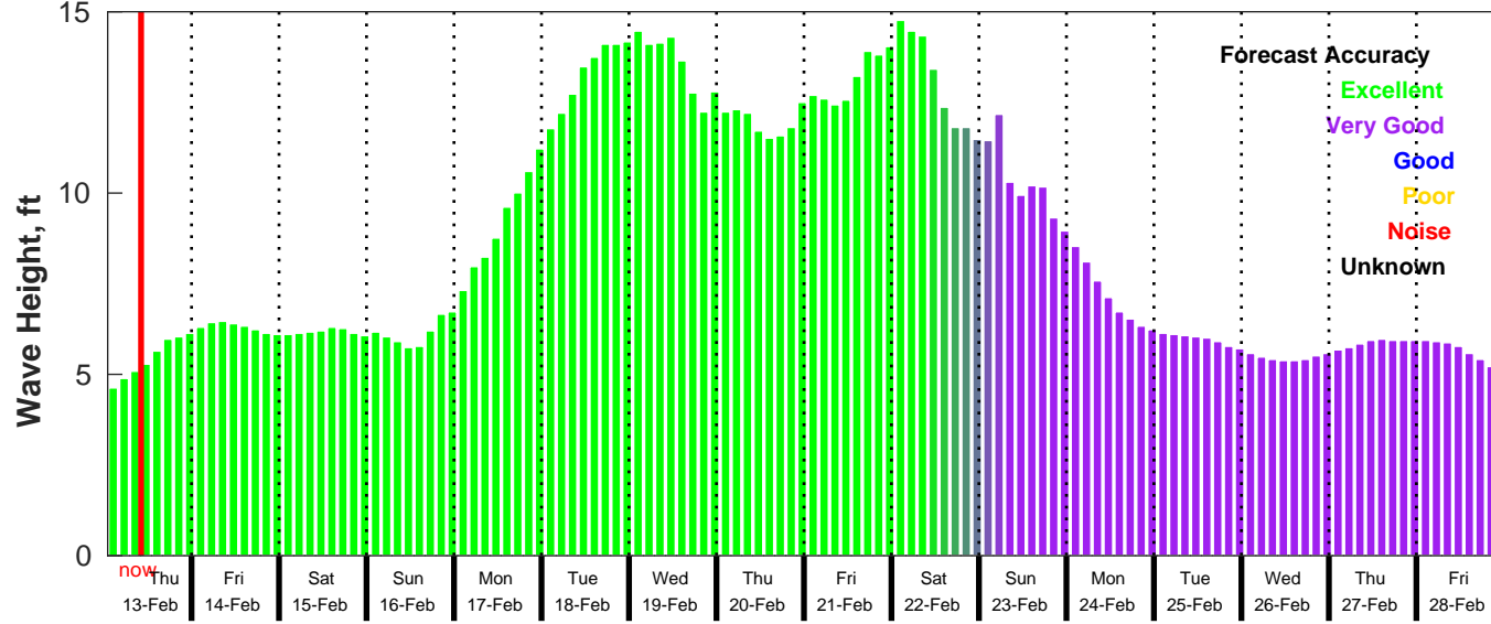
GFS Wave Forecast for NDBC 51209 from 13-Feb-2025 01:00:00 to 01-Mar-2025 01:00:00
