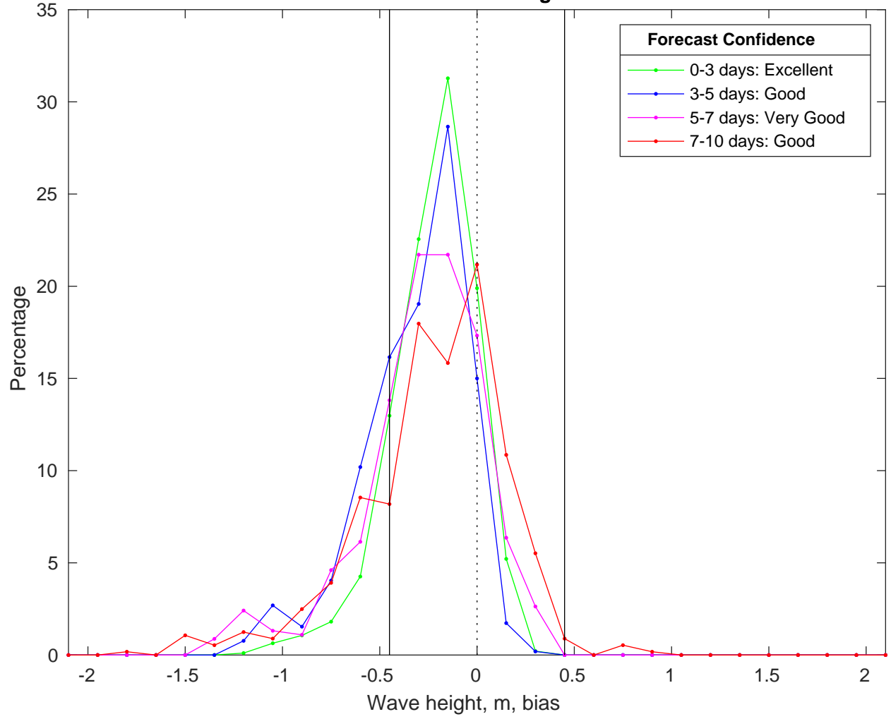
NDBC 52211 vs CMEMS Waves Bias Histogram: 13-Feb-2025
