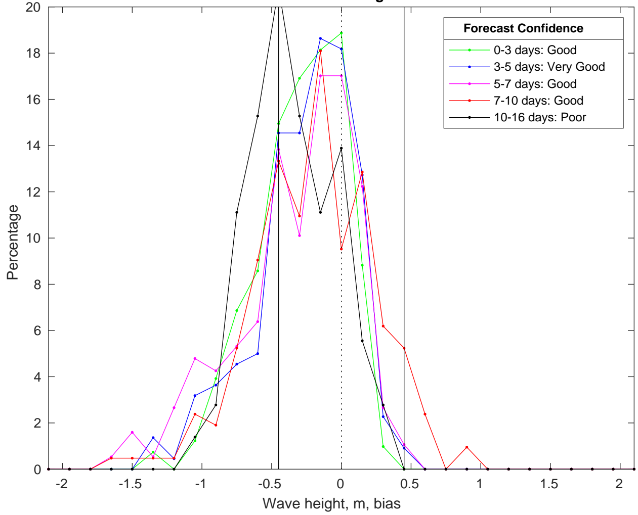
NDBC 52211 vs GFS Waves Bias Histogram: 13-Feb-2025
