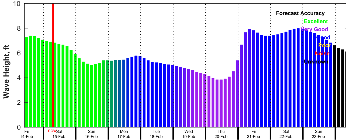
CMEMS Wave Forecast for NDBC 52211 from 13-Feb-2025 10:00:00 to 23-Feb-2025 10:00:00
