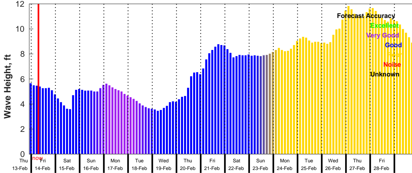
GFS Wave Forecast for NDBC 52211 from 13-Feb-2025 22:00:00 to 01-Mar-2025 22:00:00
