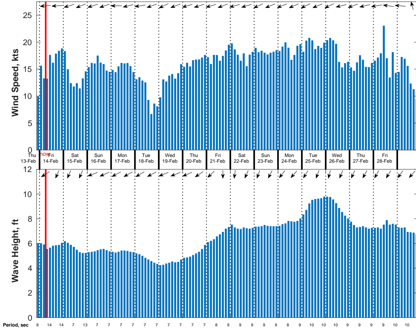
Wind & Wave Forecast for NDBC 52212 from 13-Feb-2025 21:00:00 to 01-Mar-2025 21:00:00
