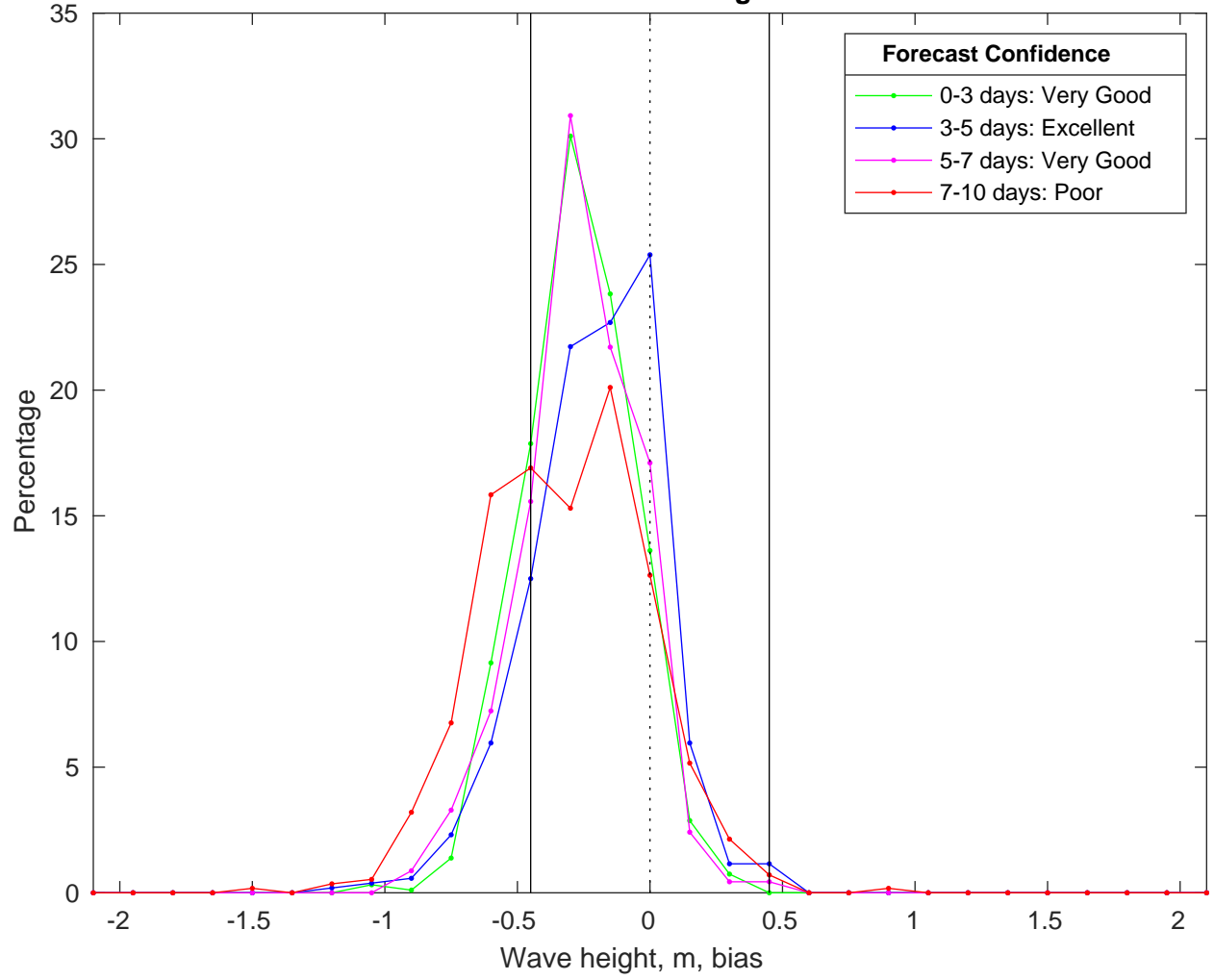
NDBC 52213 vs CMEMS Waves Bias Histogram: 13-Feb-2025
