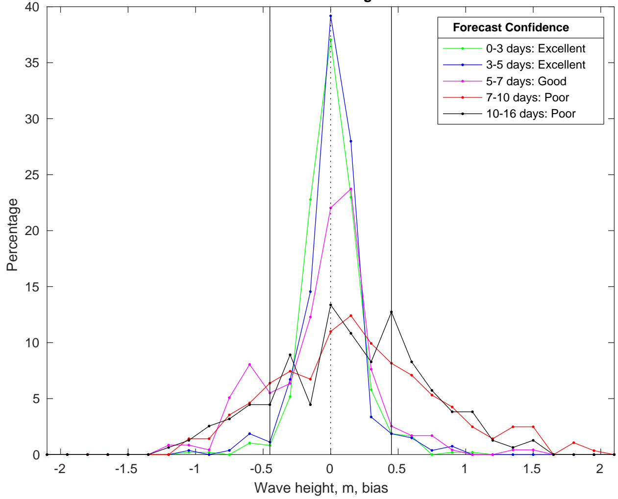
NDBC 41004 vs GFS Waves Bias Histogram: 14-Feb-2025
