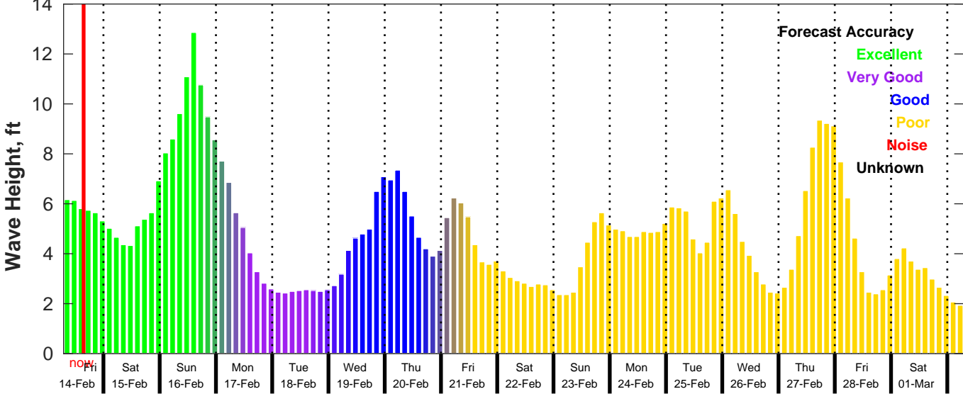
GFS Wave Forecast for NDBC 41013 from 14-Feb-2025 07:00:00 to 02-Mar-2025 07:00:00
