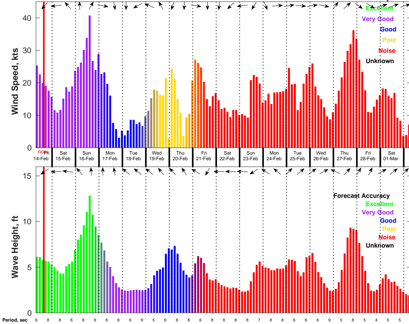
Wind & Wave Forecast for NDBC 41013 from 14-Feb-2025 07:00:00 to 02-Mar-2025 07:00:00
