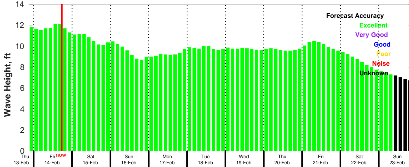
CMEMS Wave Forecast for NDBC 41040 from 13-Feb-2025 21:00:00 to 23-Feb-2025 21:00:00
