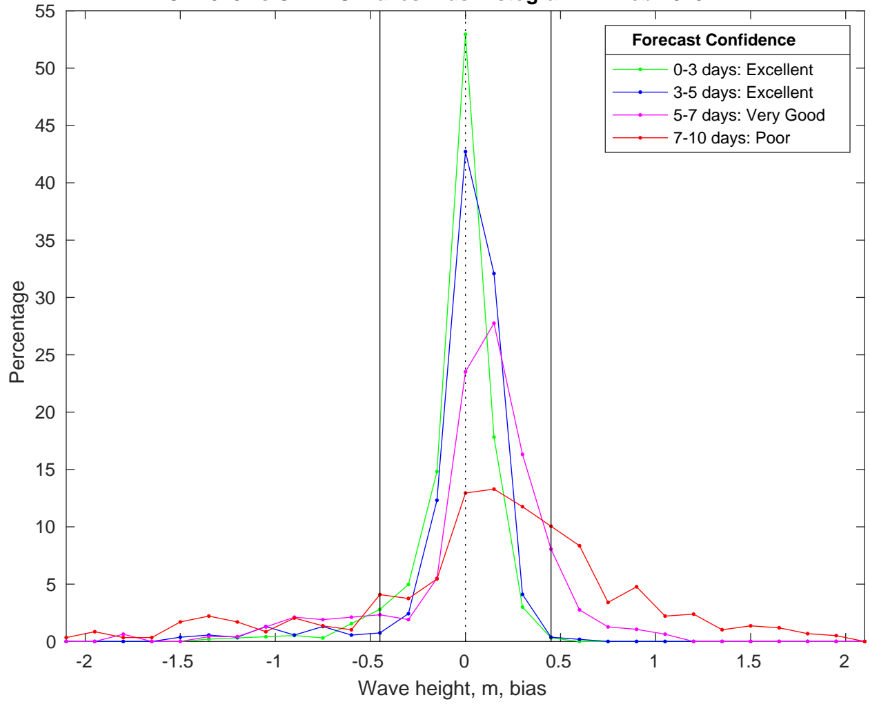
NDBC 42020 vs CMEMS Waves Bias Histogram: 14-Feb-2025
