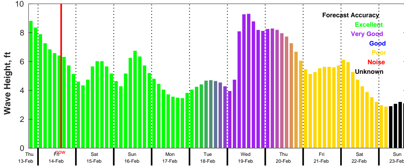
CMEMS Wave Forecast for NDBC 42020 from 13-Feb-2025 18:00:00 to 23-Feb-2025 18:00:00
