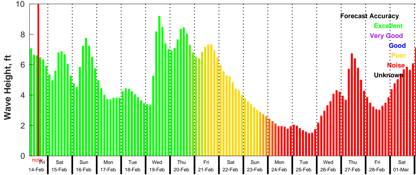
GFS Wave Forecast for NDBC 42020 from 14-Feb-2025 06:00:00 to 02-Mar-2025 06:00:00
