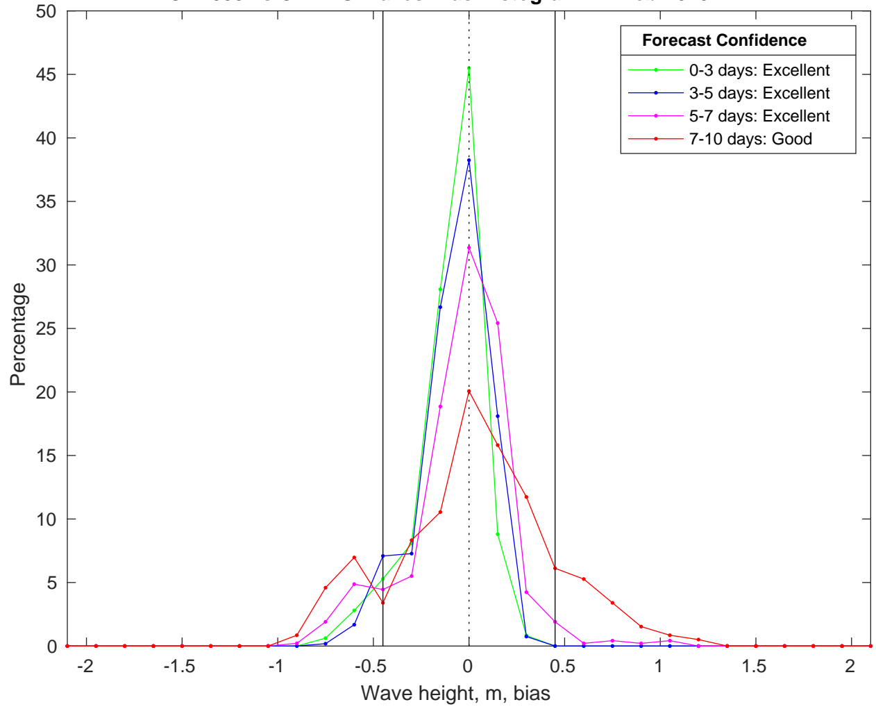
NDBC 42035 vs CMEMS Waves Bias Histogram: 14-Feb-2025
