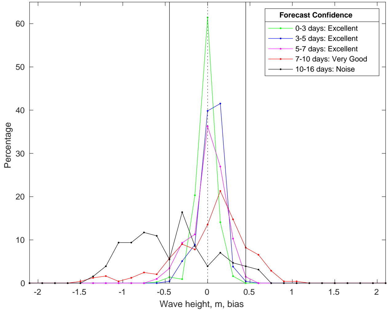
NDBC 42035 vs GFS Waves Bias Histogram: 14-Feb-2025
