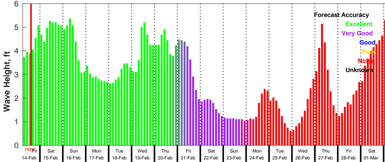
GFS Wave Forecast for NDBC 42035 from 14-Feb-2025 06:00:00 to 02-Mar-2025 06:00:00
