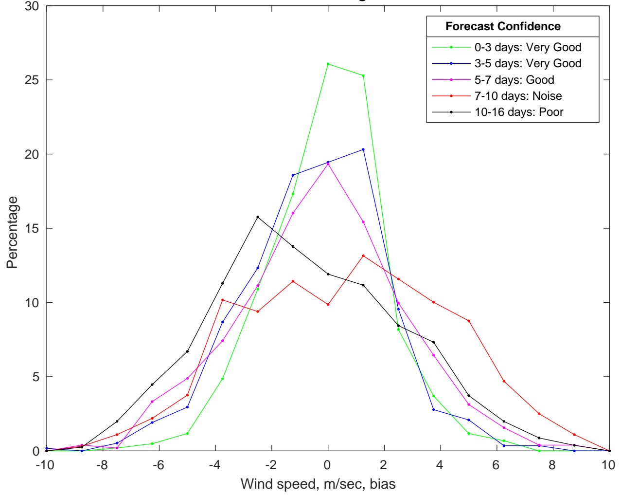
NDBC 42035 vs GFS Winds Bias Histogram: 26-Dec-2024
