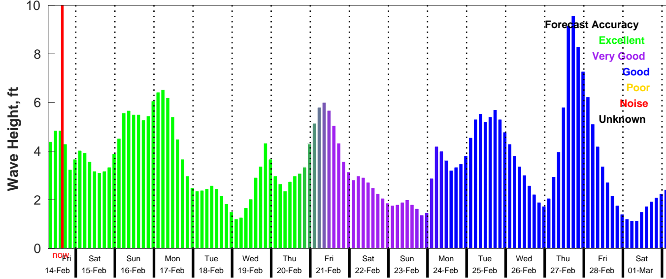
GFS Wave Forecast for NDBC 42036 from 14-Feb-2025 07:00:00 to 02-Mar-2025 07:00:00
