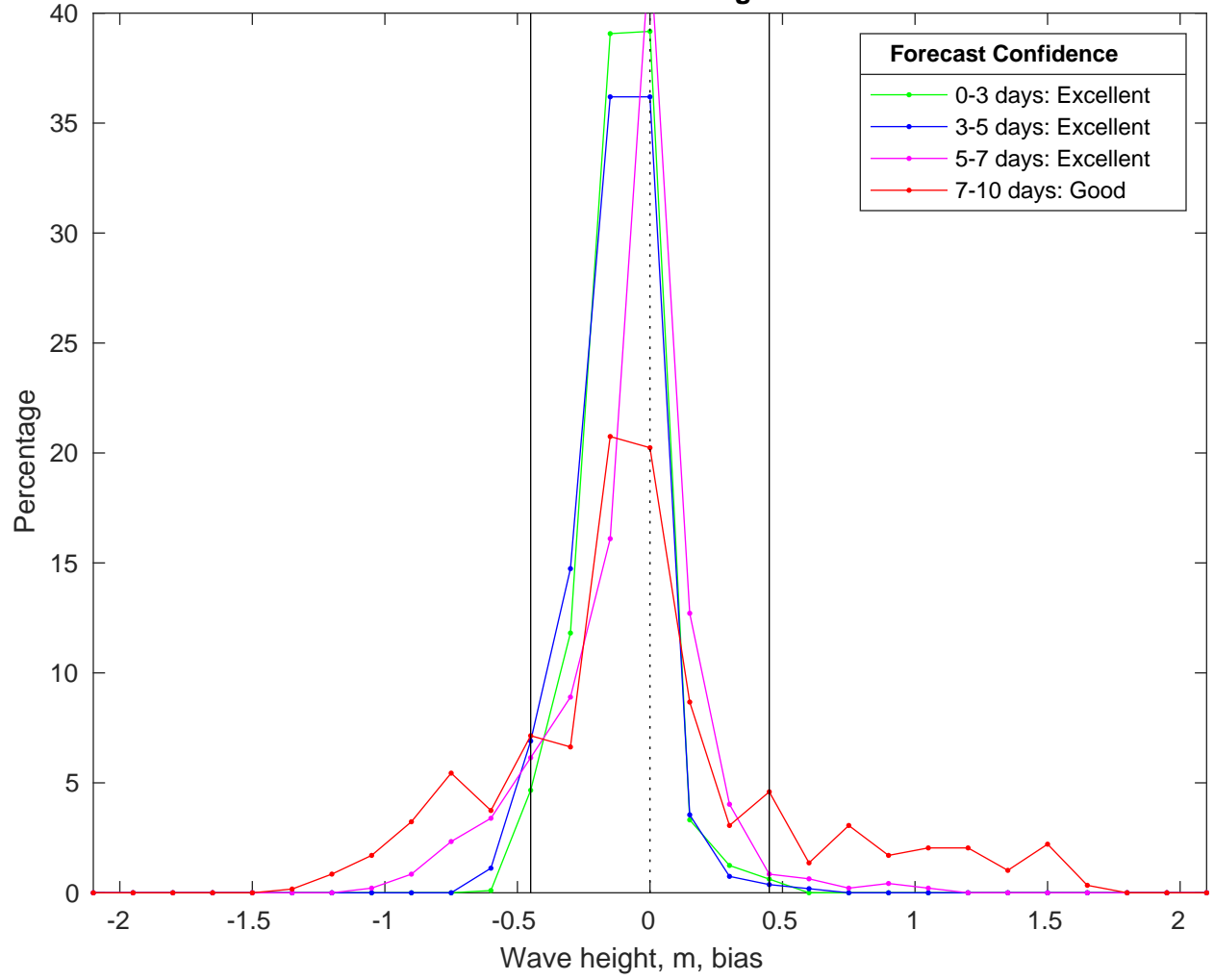
NDBC 42040 vs CMEMS Waves Bias Histogram: 14-Feb-2025
