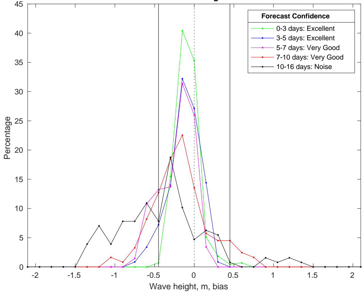
NDBC 42040 vs GFS Waves Bias Histogram: 14-Feb-2025
