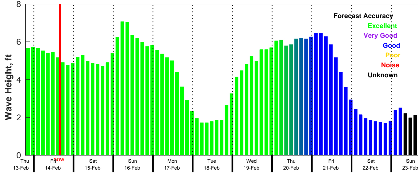
CMEMS Wave Forecast for NDBC 42040 from 13-Feb-2025 19:00:00 to 23-Feb-2025 19:00:00
