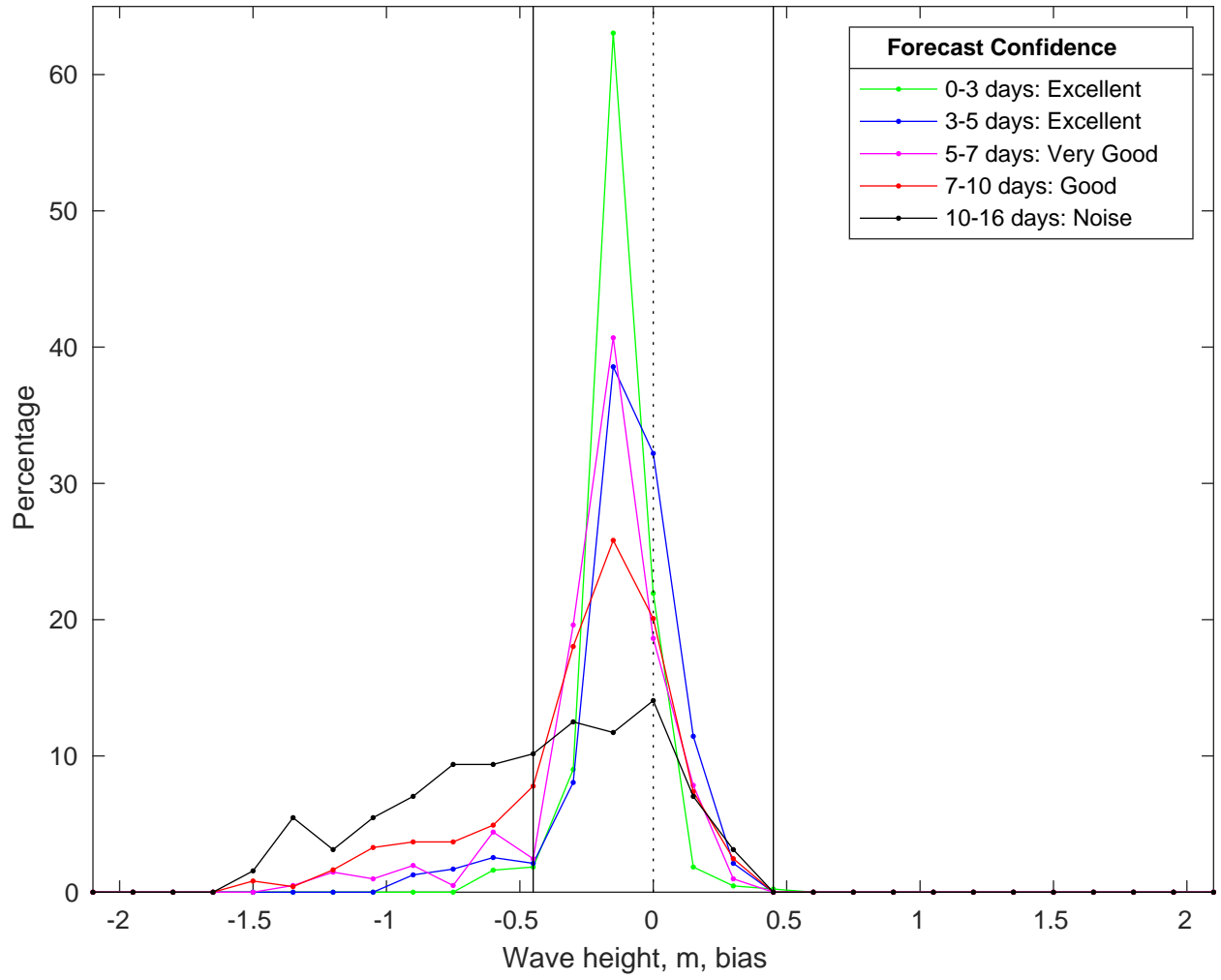
NDBC 42084 vs GFS Waves Bias Histogram: 14-Feb-2025
