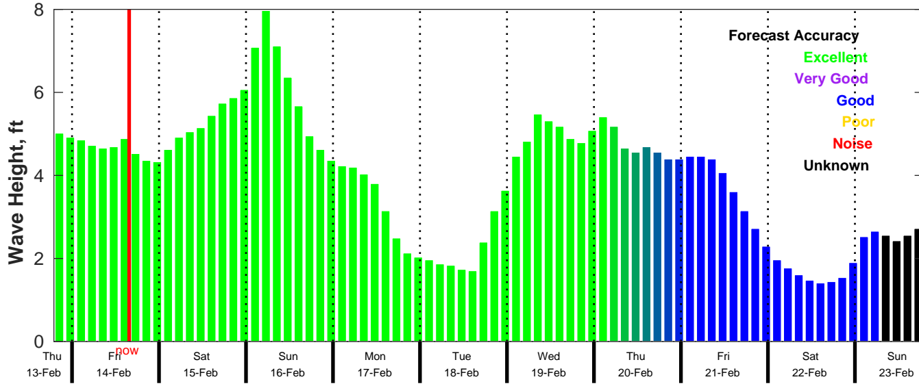
CMEMS Wave Forecast for NDBC 42084 from 13-Feb-2025 19:00:00 to 23-Feb-2025 19:00:00
