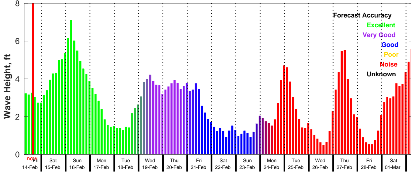
GFS Wave Forecast for NDBC 42084 from 14-Feb-2025 07:00:00 to 02-Mar-2025 07:00:00
