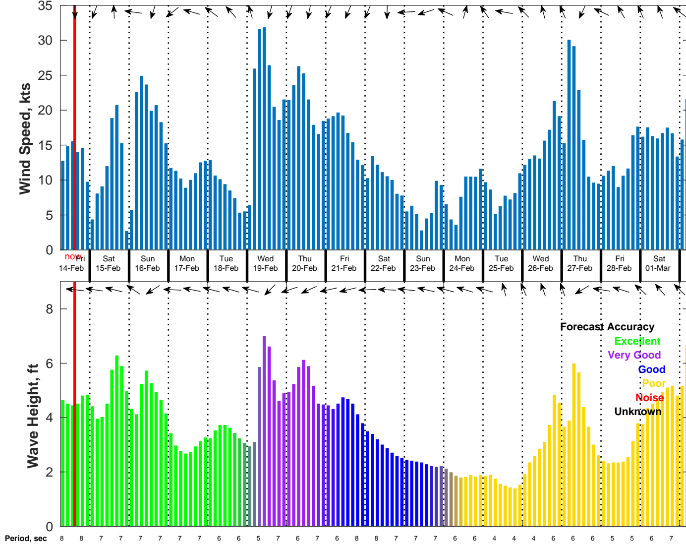
Wind & Wave Forecast for NDBC 42092 from 14-Feb-2025 06:00:00 to 02-Mar-2025 06:00:00
