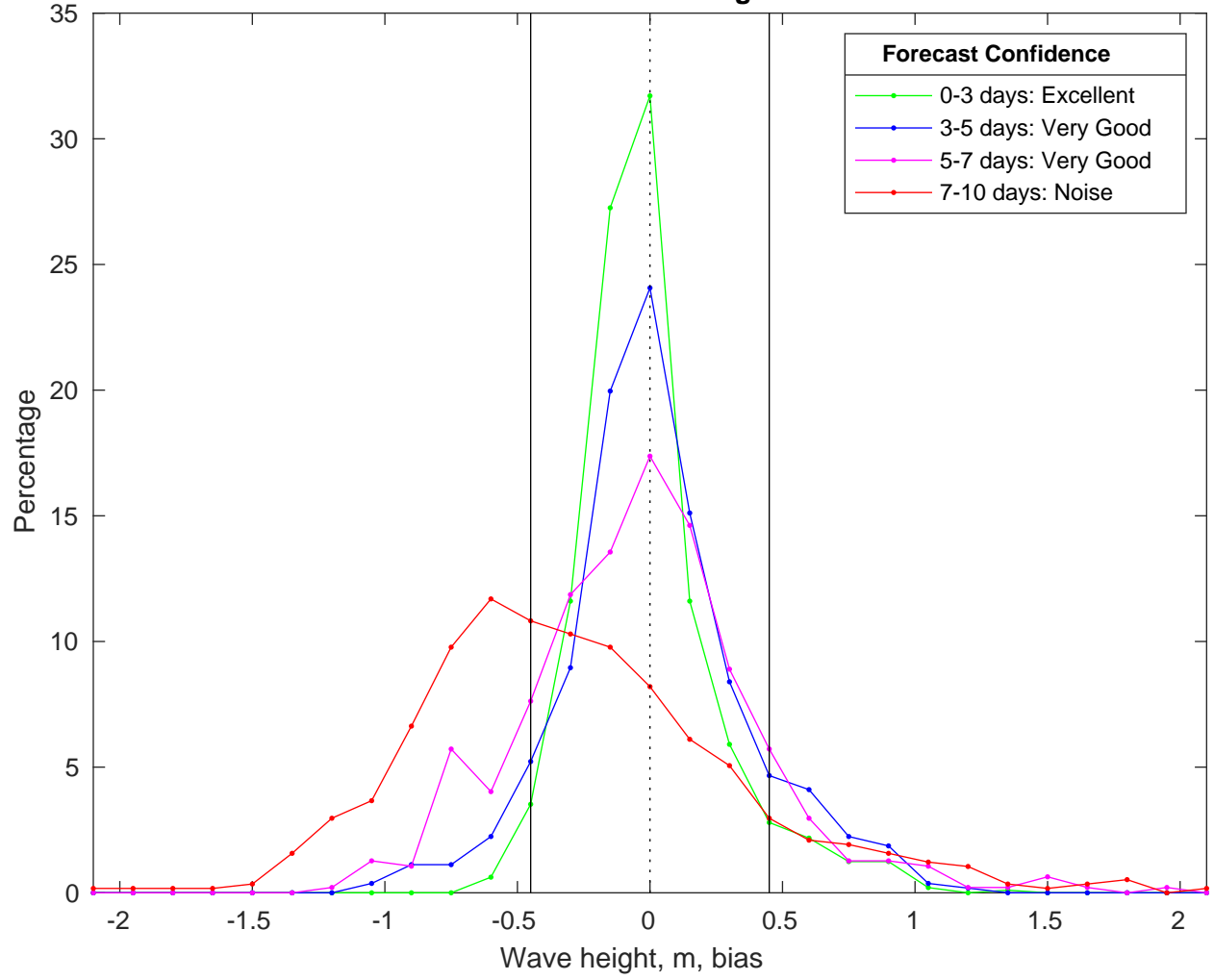
NDBC 46011 vs CMEMS Waves Bias Histogram: 14-Feb-2025
