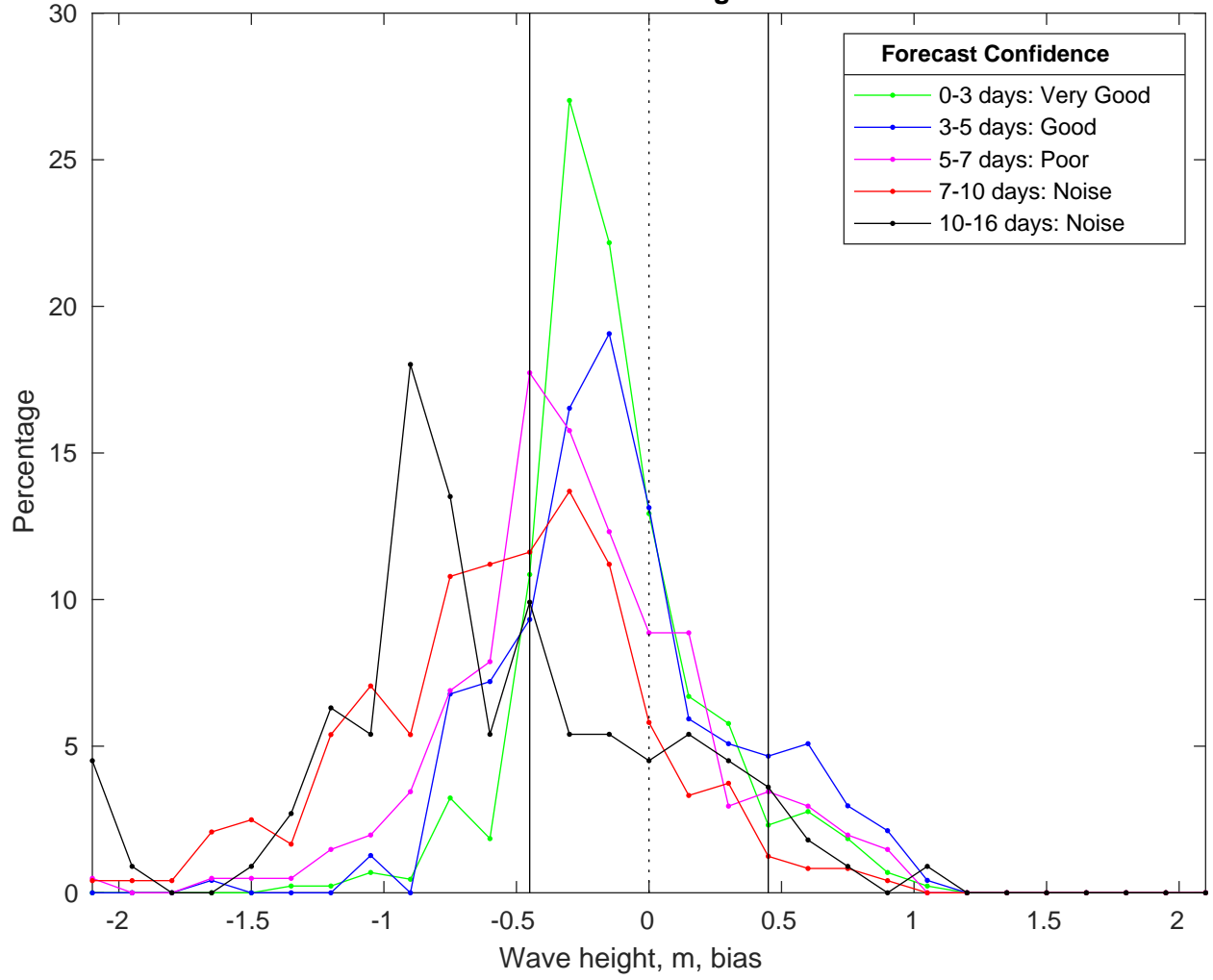
NDBC 46011 vs GFS Waves Bias Histogram: 14-Feb-2025
