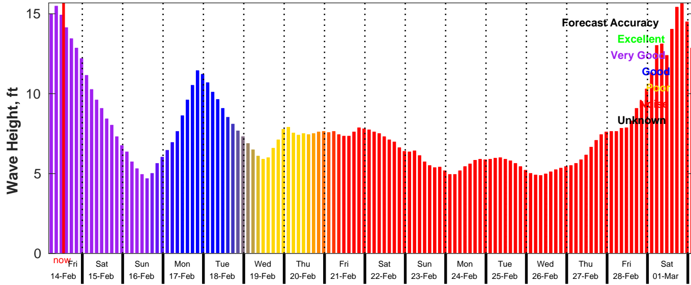
GFS Wave Forecast for NDBC 46011 from 14-Feb-2025 04:00:00 to 02-Mar-2025 04:00:00
