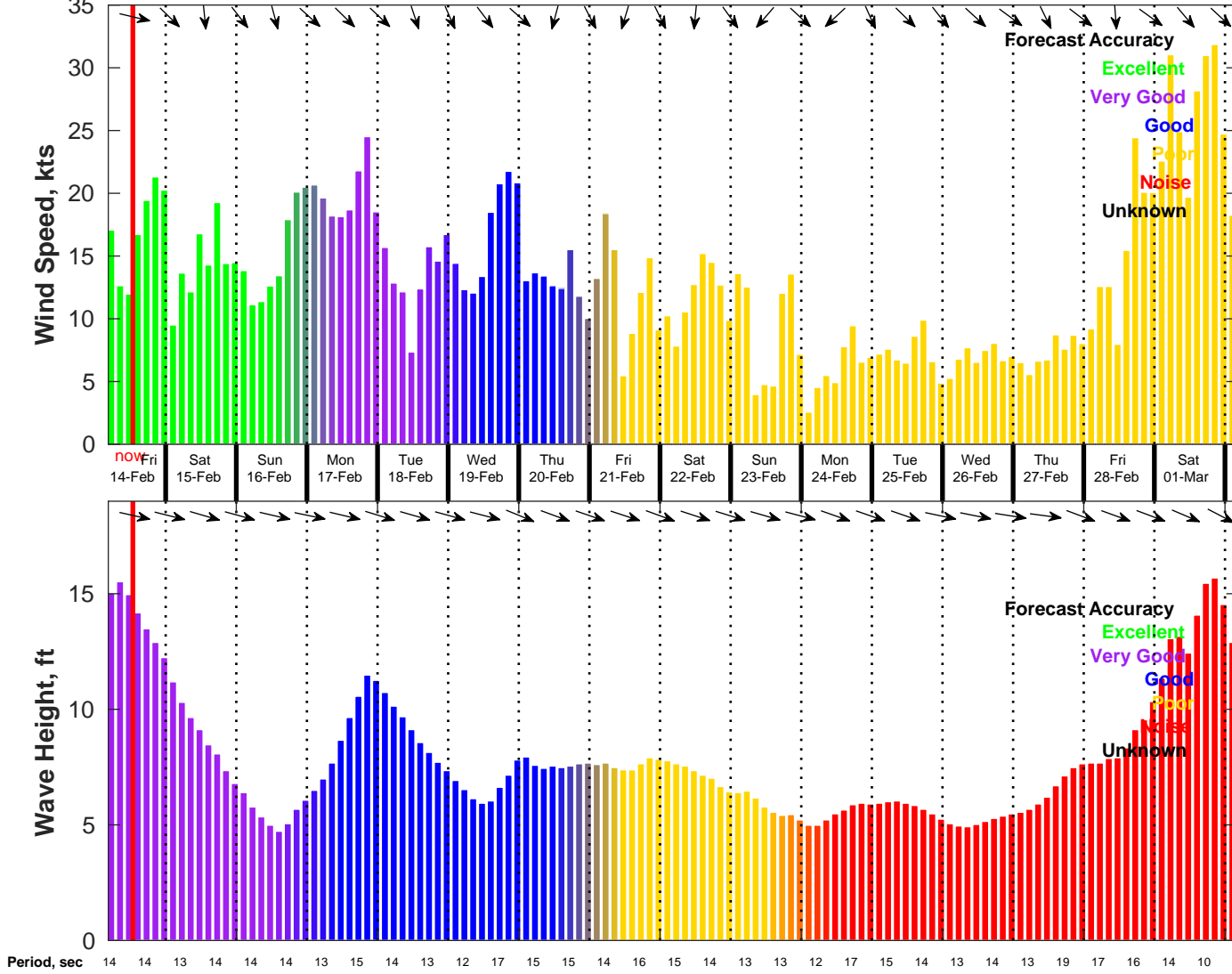
Wind & Wave Forecast for NDBC 46011 from 14-Feb-2025 04:00:00 to 02-Mar-2025 04:00:00
