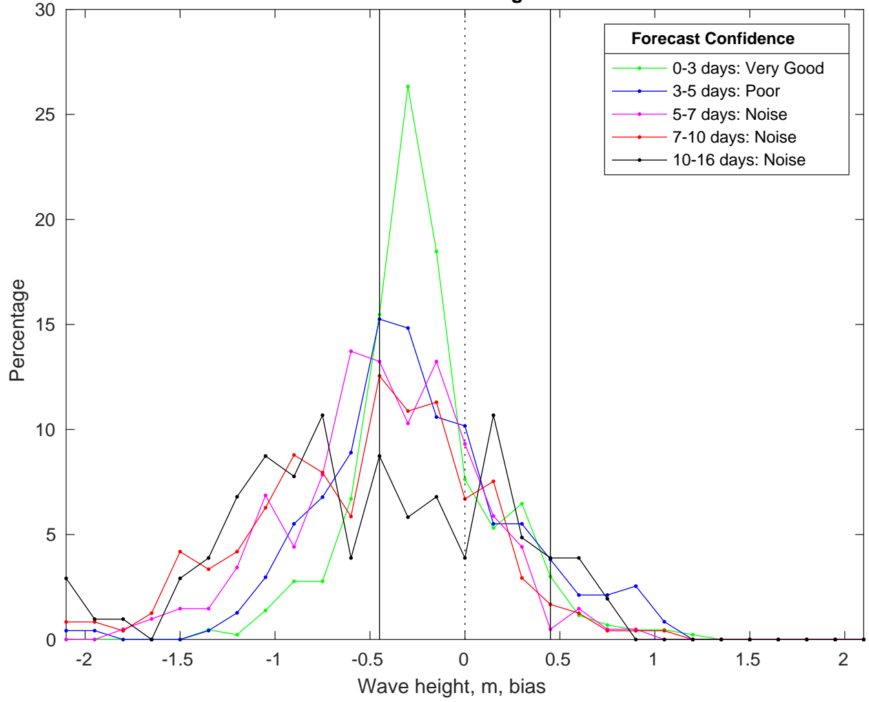
NDBC 46028 vs GFS Waves Bias Histogram: 14-Feb-2025
