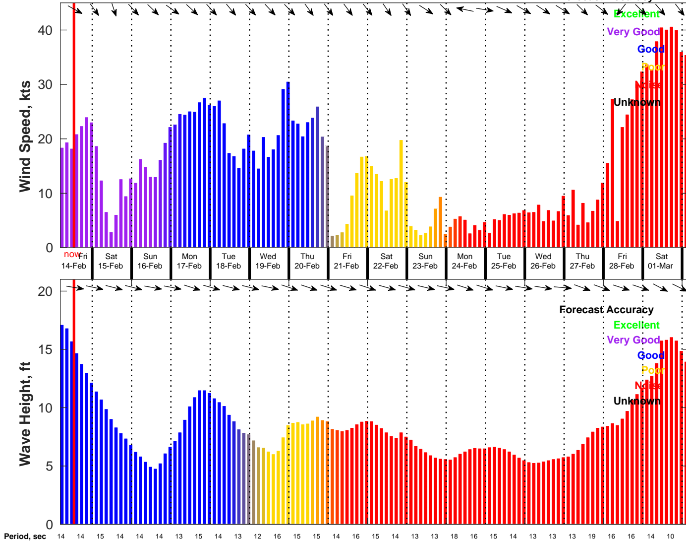
Wind & Wave Forecast for NDBC 46028 from 14-Feb-2025 04:00:00 to 02-Mar-2025 04:00:00
